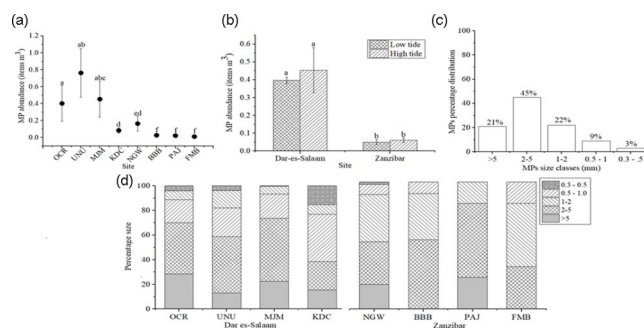
Fig. 2 Abundance and size data across study sites. (a) Average abundances of MPs ( \text{items}/\text{m}^3 ) in water samples across shown as differences between sites and (b) differences between high and low tide at Dar es Salaam and Zanzibar, respectively. Different letters indicate significant differences between data (one-way ANOVA; Tukey's HSD test, p < 0.05 ). (item/ \text{m}^3 ), mean \pm SE, n=3 ). (c) MP size distribution (in %) showing overall data for all sites combined and then (d) size breakdowns of individual sites of Dar es Salaam and Zanzibar. For site abbreviations refer to Table 1
